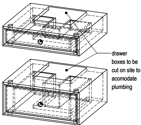
DETAIL- SPLIT DRAWERS SHOWN WITH HIDDEN LINES
